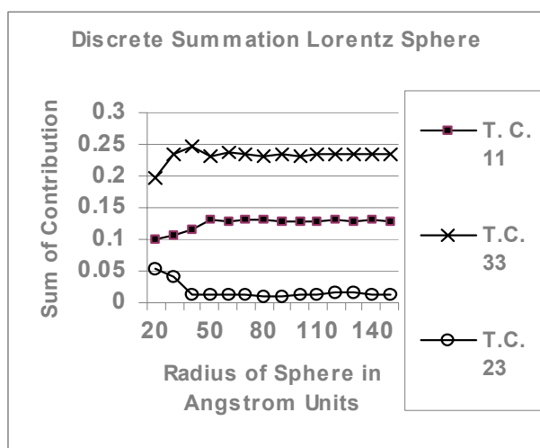
Fig.1 The graphical plot of the sum of the contributions from within Lorentz sphere as a function of the radius of the sphere. The sum reaches a Limiting Value at around 50Å. These are values reported in a M.Sc., Project (1990) submitted to N.E.H. University. T.C. stands for (shielding) Tensor Component
