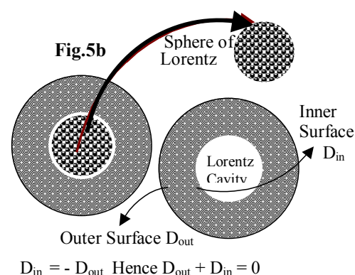
Fig.5 The various demarcations required, in an Organic Molecular Single Crystalline Spherical specimen, to Calculate the Contributions to the induced Fields at the specified site.
