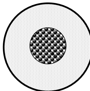
Fig.2. The demarcation (~50Å radius) of the inner Lorentz Sphere from the outer macroscopic continuum. The Lorentz Sphere is supposed to be semi-micro and the above depiction is an exaggeration for the size of the inner sphere.
